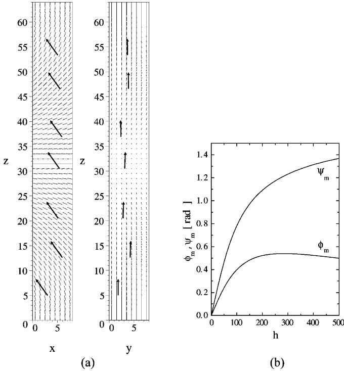
FIGURE 3 (a) Projections of the director and particle equilibrium configuration in the middle cross sections of the cell. Snapshots are taken at h_b = 10 and h = 100 ; U_p = 0.037 ( W_p = 5 \times 10^{-4} erg \text{cm}^{-2} ). (b) The angle of maximum deviation of the nematic director inside the cell \phi_m and the corresponding angle of the ferroparticle \psi_m vs the normalized magnetic field calculated with the continuum theory of FN [8] for W_p = 0.01 erg \text{cm}^{-2} .
